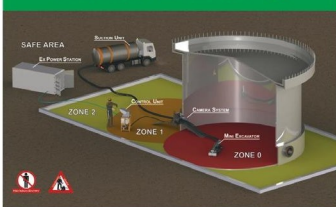
Robotic Tank Cleaning
